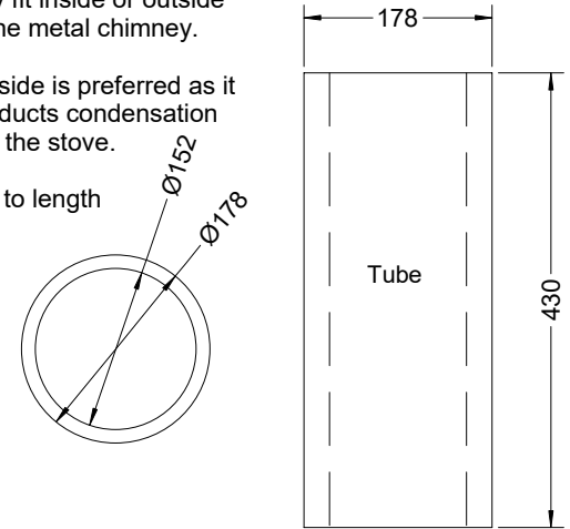
Clay Chimney Connector
