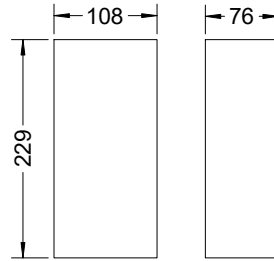
High Temp Solid Brick
