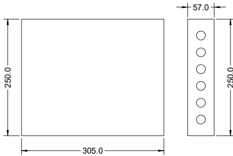
Perforated Clay Tile (optional) Not normally used
